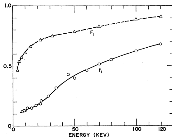
FIG. 3. Ratio f_1 = N_H / (N_H + N_{H_2}) , where N_H and N_{H_2} are, respectively, the fluxes of H atoms and H 2 molecules in the composite neutral beam entering collision chamber T_2 during the H 2 primary measurements. Ratio F_1 = \sigma_H / (\sigma_H + \sigma_{H_2}) , where \sigma_H and \sigma_{H_2} are, respectively, the cross sections for production of fast H and H 2 secondaries in collisions of fast H 2 + ions with H 2 molecules. F_1 is calculated from the experimental data of Ref. 1.
