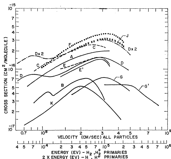
FIG. 7. Curve A: \sigma_{H_2^+} the cross section for conversion of fast H 2 molecules to H 2 + ions from Fig. 4. Curve B: \sigma_{H^+} the cross section for conversion of fast H 2 molecules to H + ions from Fig. 4. Curve C gives the sum of \sigma_{H^+} and \sigma_{H_2^+} which equals the total cross section for electron loss from fast H 2 molecules. Curves D and D×2 are, respectively, 1 and 2 times the cross section \sigma_{0,1} for electron loss from H atoms from Fig. 2. Curve E: ionization of H 2 by H primaries, including \sigma_{1,-1} the ion production due to electron capture by the primary ions from Schwitzke (Ref. 9). Curve E': curve E minus \sigma_{1,-1} from Fig. 2. Curve F: cross section for free electron production in H 2 + +H 2 collisions from Afrosimov (Ref. 15). Curve G and G' are, respectively, the results of Guidini (Ref. 16) and Sweetman (Ref. 2) for electron loss from H 2 + ions in collision with H 2 . Curve F with curve G subtracted to give cross section for electron removal from H 2 when struck by H 2 + . Curve K: cross section for production of slow H + ions in collision of H 2 + with H 2 from Afrosimov (Ref. 15). A portion of curve D×2 between abscissa values 1.5 and 3 \times 10^8 cm/sec was deliberately left out to avoid confusion with curve J.
